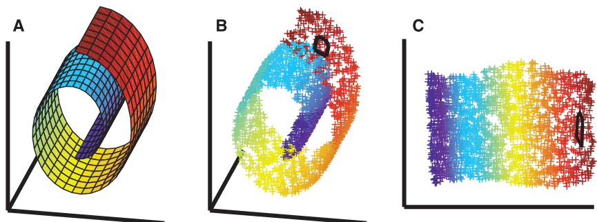
Fig. 1. The problem of nonlinear dimensionality reduction, as illustrated ( 10 ) for three-dimensional data (B) sampled from a two-dimensional manifold (A). An unsupervised learning algorithm must discover the global internal coordinates of the manifold without signals that explicitly indicate how the data should be embedded in two dimensions. The color coding illustrates the neighborhood-preserving mapping discovered by LLE; black outlines in (B) and (C) show the neighborhood of a single point. Unlike LLE, projections of the data by principal component analysis (PCA) ( 28 ) or classical MDS ( 2 ) map faraway data points to nearby points in the plane, failing to identify the underlying structure of the manifold. Note that mixture models for local dimensionality reduction ( 29 ), which cluster the data and perform PCA within each cluster, do not address the problem considered here: namely, how to map high-dimensional data into a single global coordinate system of lower dimensionality.
